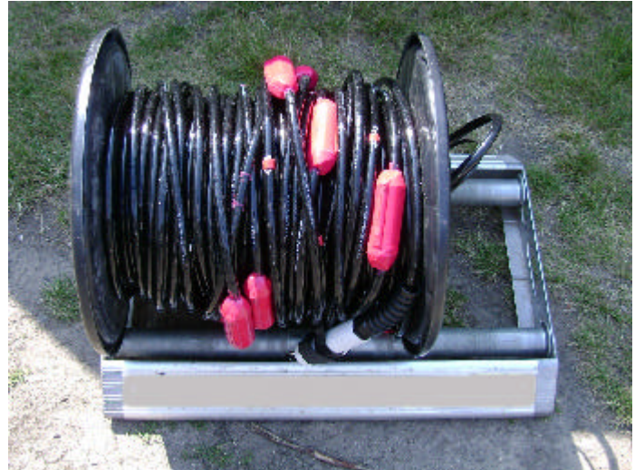
BHC4 on drum and with spooler device
