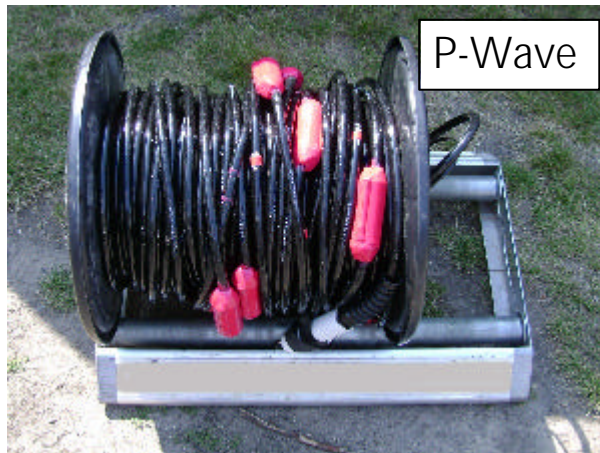
Hydrophone Strings with 12, 24 or 48 channels
