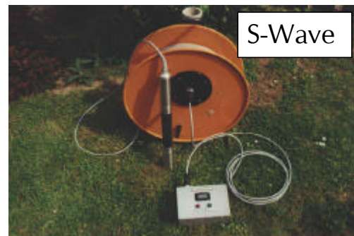
3C-Geophone with magnetic compass and pneumatic clamping
