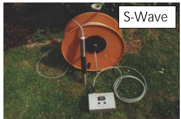
3C-Geophone with magnetic compass and pneumatic clamping
